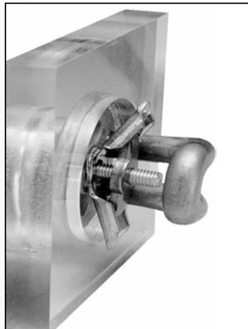
V-Loc™ clamp spreads outward as locking bolt it tightened.
